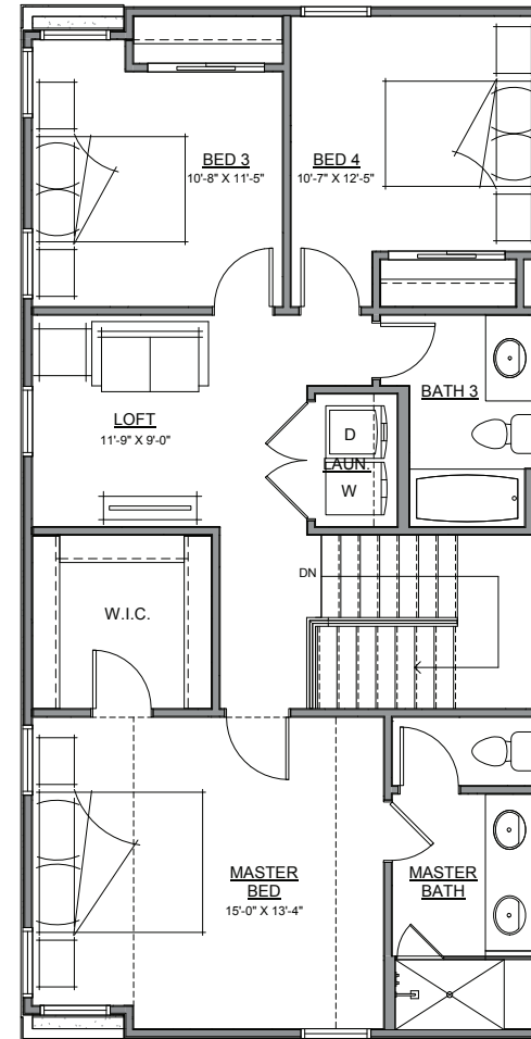
THIRD FLOOR
