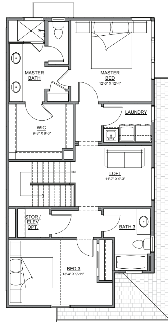
THIRD FLOOR
